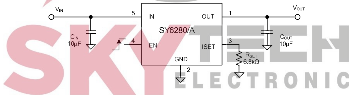
Figure 1. Schematic Diagram(1A current limit)
